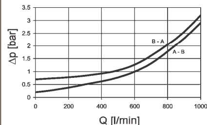
\Delta p optimized DFFX 330, 500, 660, 990, 1320
