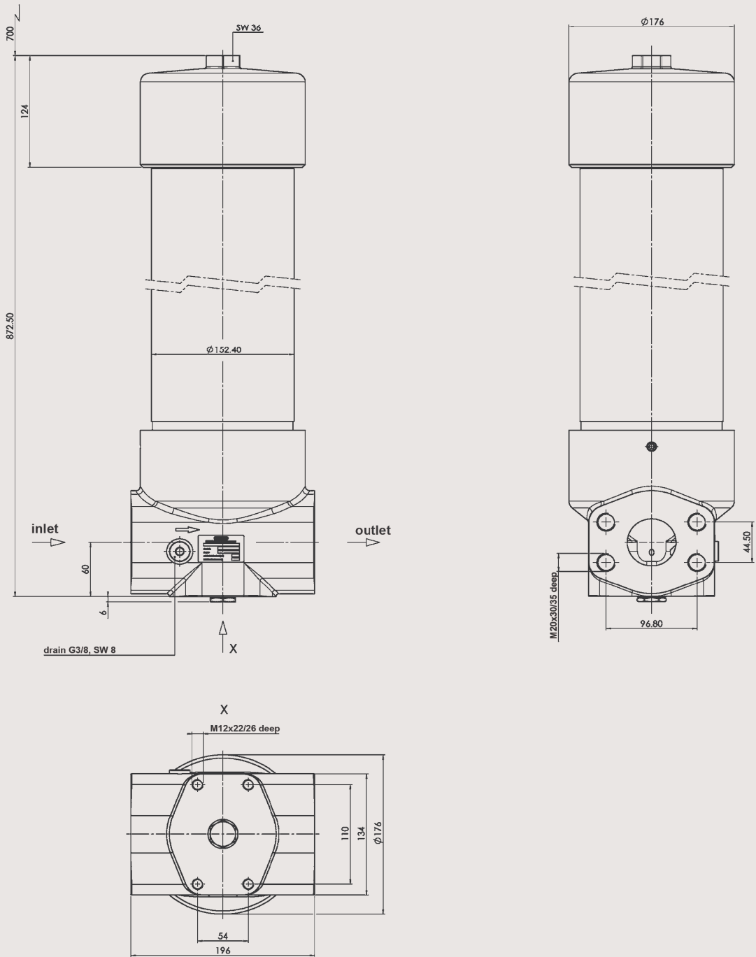
DF 1500...3.X (element top-removable)
