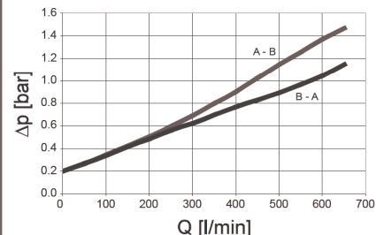
\Delta p optimized DFFX 330, 500, 660, 990, 1320
